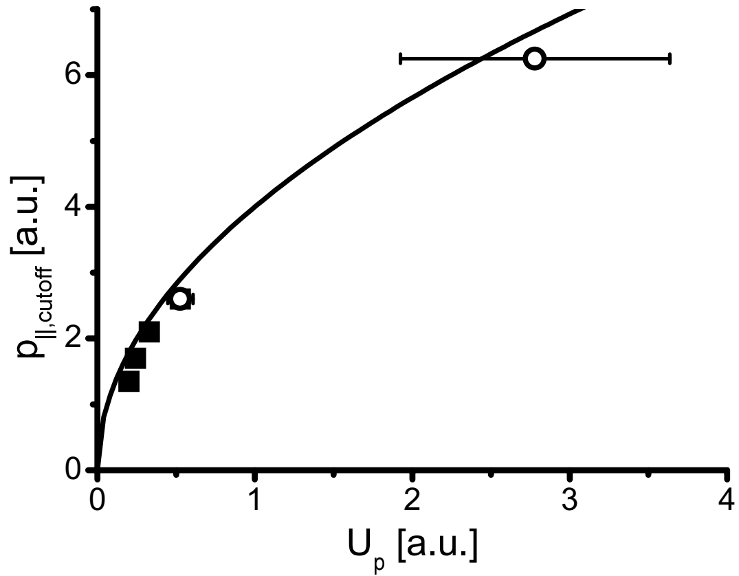
Figure 3. The dependence of the "cutoff" of the doubly charged ion momentum distributions f(p_{||}) on the light intensity determined for \text{Ar}^{++} (squares) and \text{Ne}^{++} (open circles). The line gives the calculated maximum momentum ( 4\sqrt{U_p} ) which can be imparted on the ion by the light pulse.
