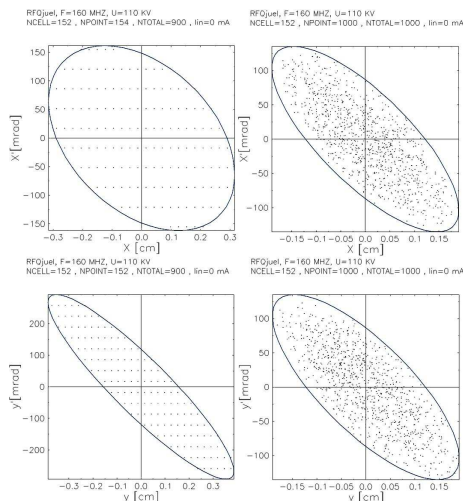
Figure 4: Input distribution and acceptance of the RFQ.
