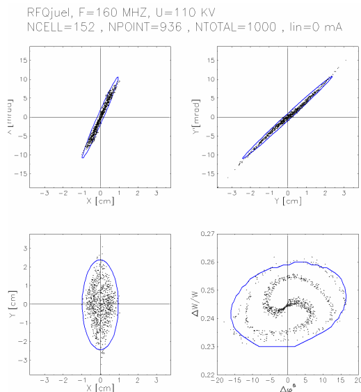
Figure 8: Beam distribution after the matching section.
