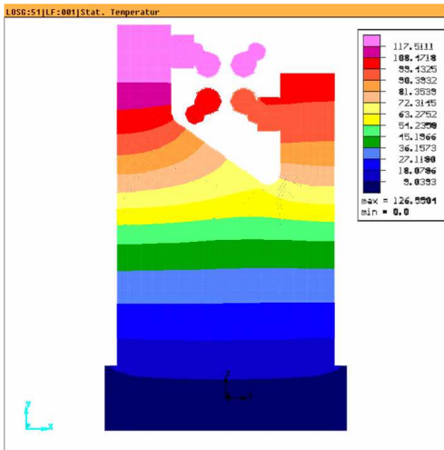
Figure 3: Temperature distribution in an RFQ stem without cooling calculated with ISAFEM.
