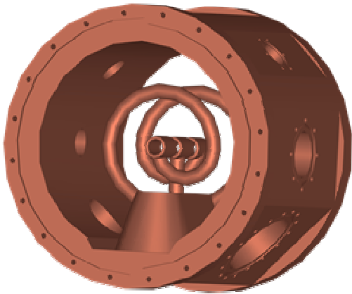
Figure 7: drawing of the spiral loaded cavity.
