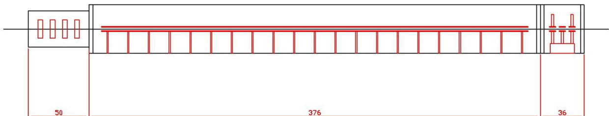
Figure 1: Overview of RFQ and Booster
