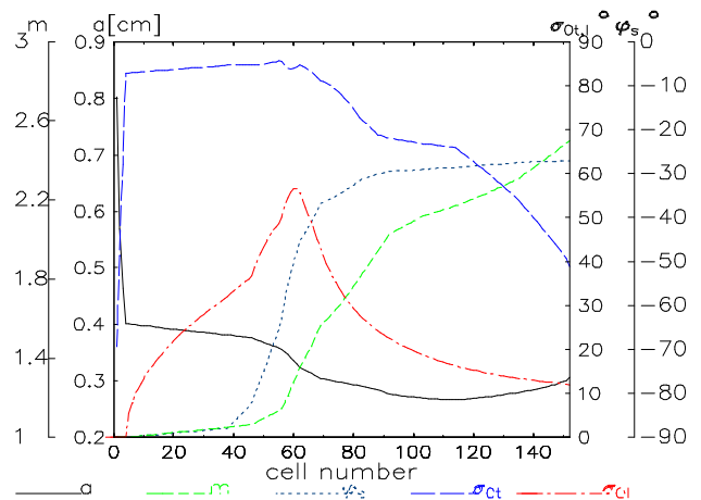
Figure 2: Design parameters of the RFQ
