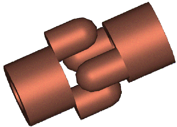
Figure 9: Schematic drawing of an accelerating gap with quadrupoles
