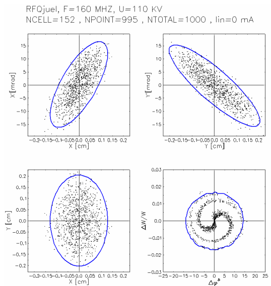
Figure 6: Output distribution of the RFQ.
