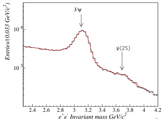
Figure 5. The e^+e^- invariant mass spectrum.
