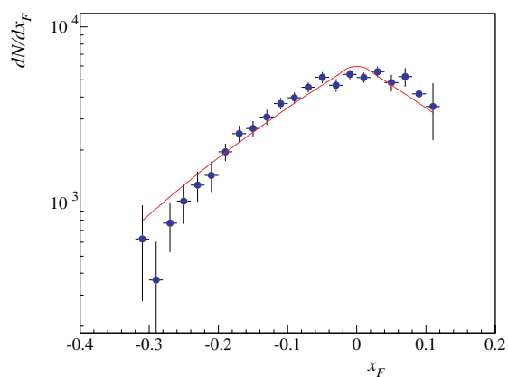
Figure 3. The x_F distribution of J/\psi \rightarrow e^+e^- .
