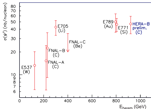
Figure 6. The \psi(2S) cross section as function of the proton beam energy.
