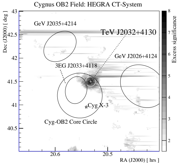
Figure 5. TeV significance map of the Cygnus OB2 field, including GeV error ellipses and positions of known sources [15].
