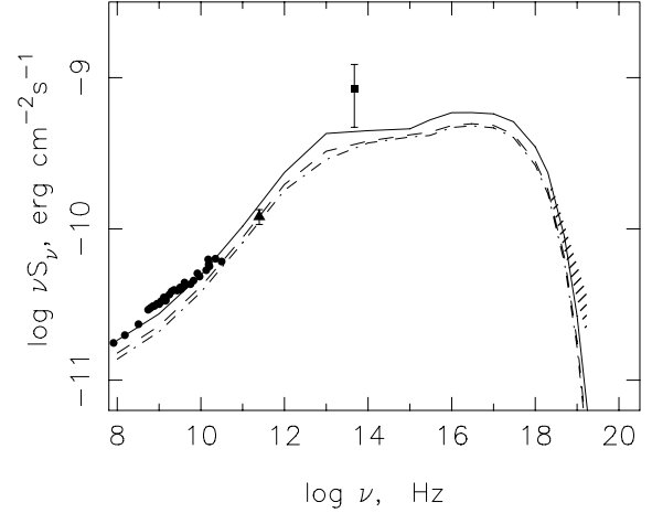
Figure 9. Radio and X-ray emission from Cas A, observed in different years. The model curves correspond to the epochs 1970, 2003 and 2022 [24].
