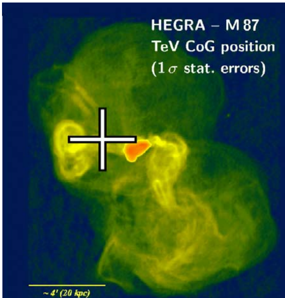
Figure 1. Radio image of M87 and its jet in the Virgo cluster at 90 cm. The cross (statistical 1\sigma errors) marks the position of the TeV \gamma -ray excess detected by HEGRA [18].
