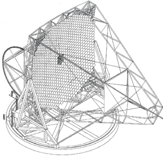
Figure 12. Configuration of a 600m 2 Cherenkov telescope, with steel structure and parabolic mirror support, for a 5 km altitude array. Not yet adapted to high altitude conditions.
