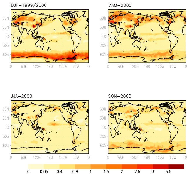
Fig. 1. Seasonal averages of H_2SO_4 concentrations in mass mixing ratios (MMR) at 700 hPa (multiplied by 10^{12} ).
