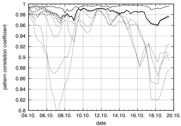
Fig. 6. Six-hourly time-series of mslp pattern correlation coefficients between DWD and NCEP-NCAR analysis data (solid) and DWD analysis data and CLM simulation data, nudged (dashed) and non-nudged (dotted) over all maritime grid cells from 4 to 20 October 1993.
