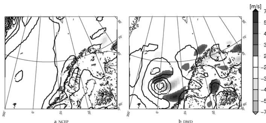
Fig. 7. Bandpass filtered mean sea level air pressure (hPa) and 10 m wind speed from NCEP–NCAR analysis data and from DWD analysis data at 0600 UTC 15 October 1993.
