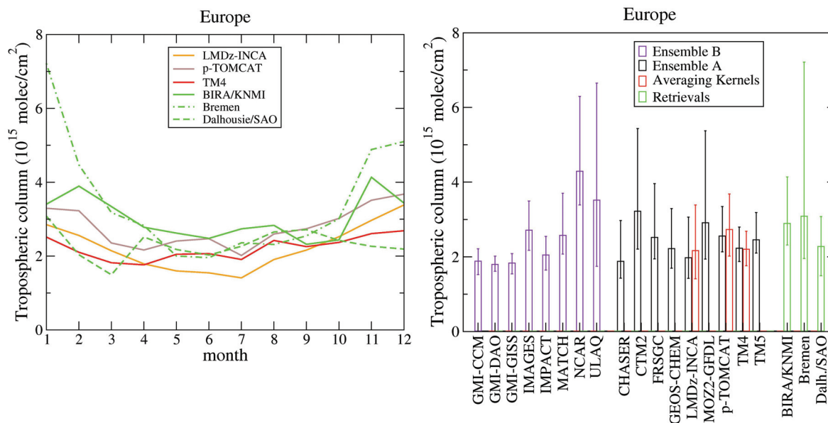
Figure 18: Left: Seasonal cycle in the tropospheric \text{NO}_2 column density over Europe. Shown are the monthly values calculated by application of the averaging kernels to the daily 3-dimensional output fields from LMDz-INCA, p-TOMCAT and TM, together with the corresponding retrievals (green lines). Right: Annual mean tropospheric \text{NO}_2 column density together with the minimum and maximum monthly mean values for Europe. Results calculated from the daily model columns ('Ensemble A', 'Ensemble B') or the daily 3-dimensional output fields ('Averaging Kernels'), are compared to the retrieval data.
