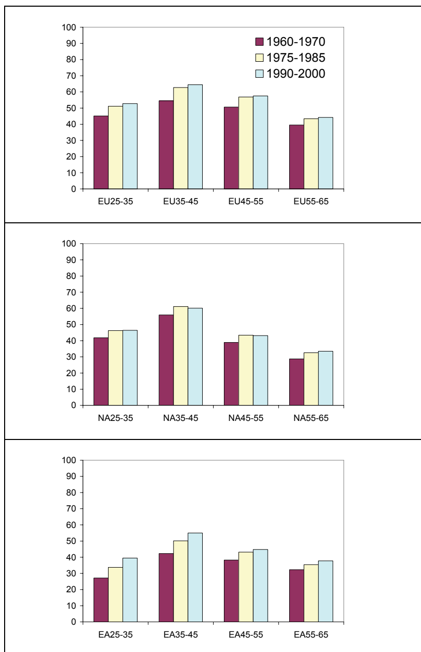
Figure 27: Decadal mean summertime boundary layer (0-1 km) ozone concentrations over Europe (top), North America (center) and East Asia (bottom) as derived from the mean results of the three individual models
