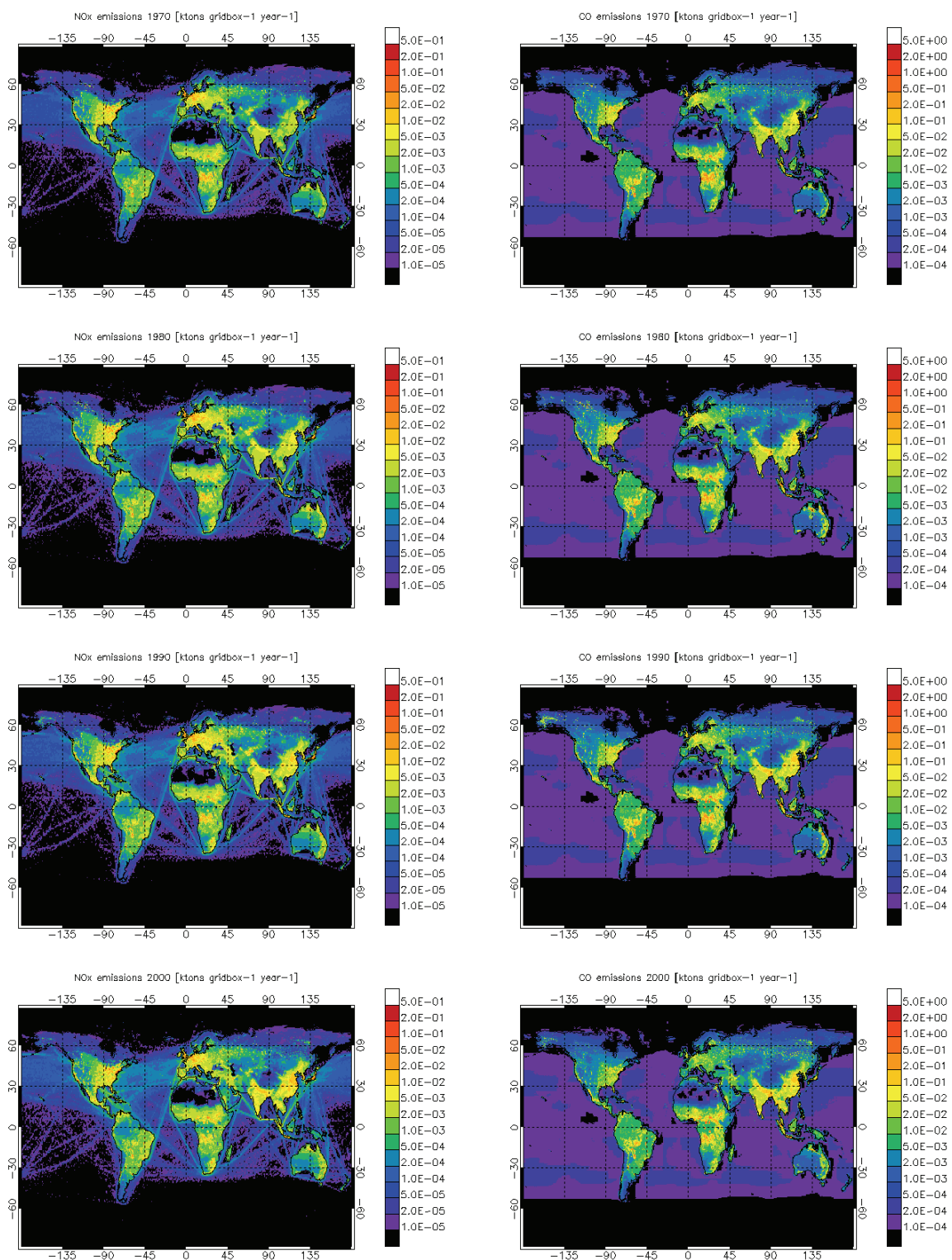
Figure 9: Spatial distribution of \text{NO}_x (left) and \text{CO} (right) emissions from the RETRO inventory for the years 1970, 1980, 1990 and 2000 (top to bottom). These figures contain all RETRO surface emissions (including wild fires and natural sources, but without aircraft and lightning \text{NO}_x emissions)
