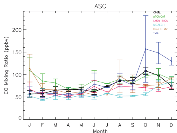
Figure44: Year-1997 Surface CO concentrations at Ascension Island (ASC) [from D3-2]. Model results from a preliminary set-up
