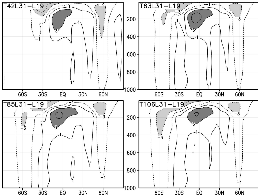
FIG. 11. As in Fig. 9, but for differences L31 - L19.
