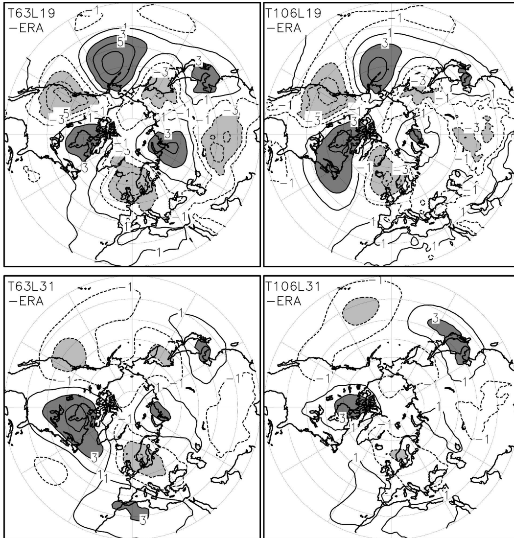
FIG. 17. As in Fig. 16, but for differences between model simulations and ERA-15. Contours are \pm 1, 3, 5, and 7 \text{ dam} . Negative biases ( < -3 \text{ dam} ) are emphasized by light shading, positive biases ( > 3 \text{ dam} ) by dark shading.
