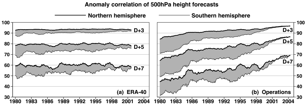
Figure 14. Twelve-month running mean anomaly correlations (%) of 3-, 5- and 7-day 500 hPa height forecasts for the extratropical northern and southern hemispheres: (a) 12 UTC ERA-40 forecasts from January 1980 to August 2002; (b) operational 12 UTC ECMWF forecasts from January 1980 to April 2005. The shading shows the difference in scores between the two hemispheres at the forecast ranges indicated. (See appendix A for acronyms.)
