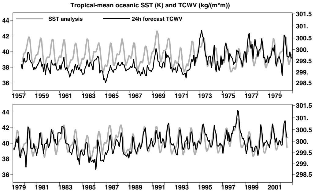
Figure 17. Monthly averages from 1957 to 2002 of 24 h forecast TCWV (black; \text{kg m}^{-2} ; left-hand scale) averaged over tropical oceans, and the mean tropical SST used in ERA-40 (grey; K; right-hand scale). The temperature scale is linear in saturation specific humidity for a reference surface pressure of 1013.25 hPa, and chosen to make the mean and standard deviation of the two time series equal for the SSM/I period from July 1987 onwards. (See appendix A for acronyms.)
