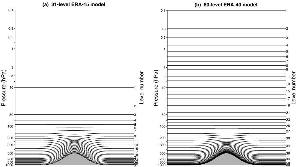
Figure 4. The distribution of full model levels at which the basic prognostic variables are represented for: (a) ERA-15 and (b) ERA-40.
