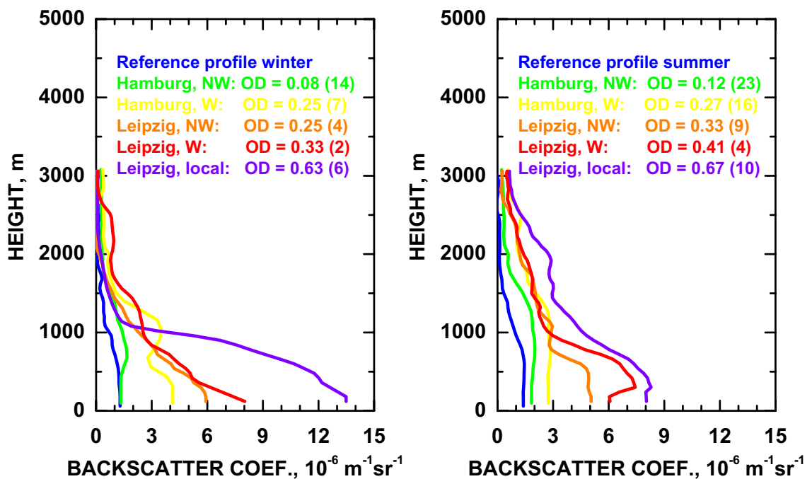
Figure 53: Mean backscatter-coefficient profiles for different flows obtained at Leipzig and Hamburg. The reference profiles for clean conditions are shown for comparison. The optical depth (OD) and the number of averaged measurements for each profile are given in the legend.
