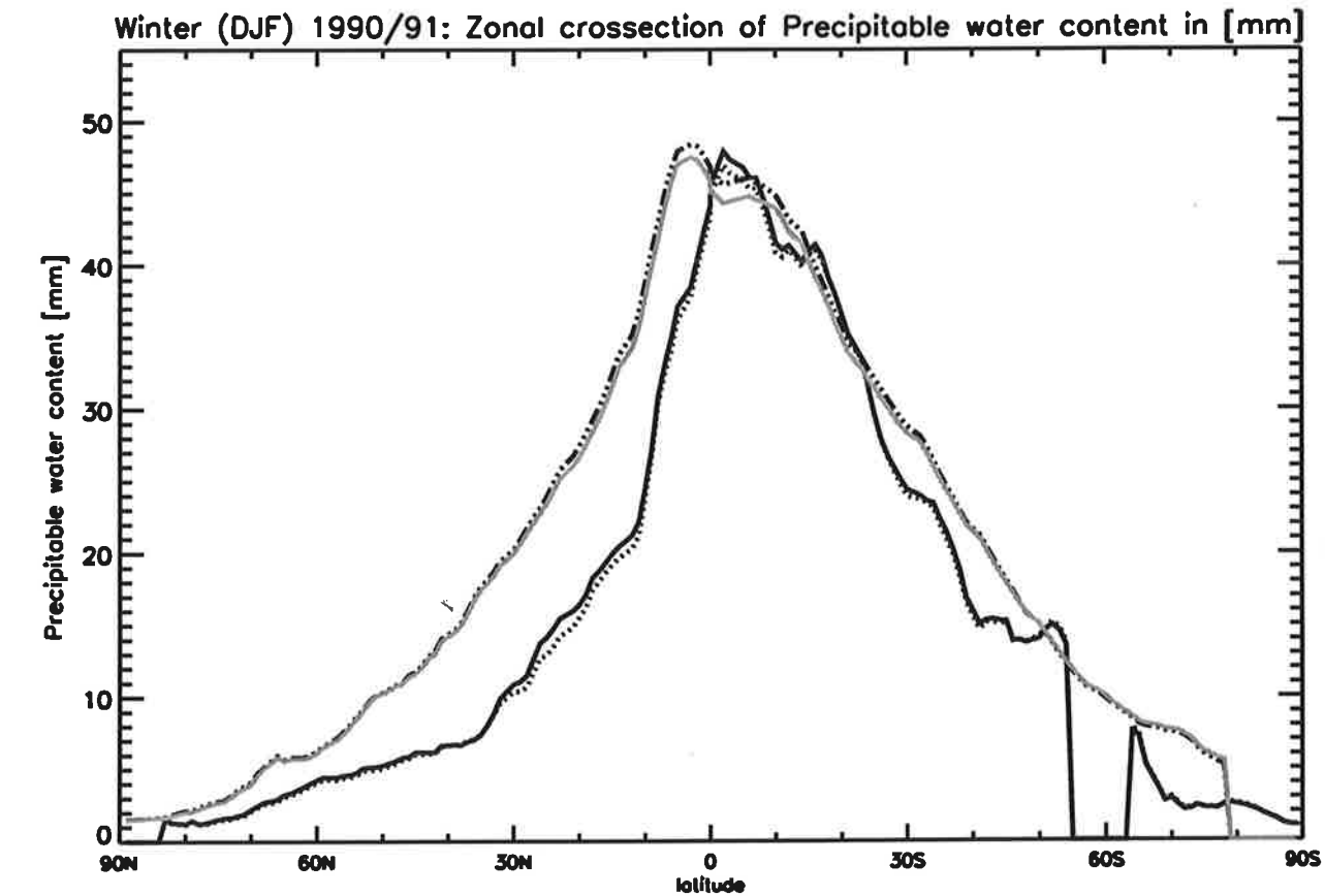
— ERA40 - land ····· Exp. b02d - land -·-·- ERA40 - ocean — Exp. b02d - ocean (b)
