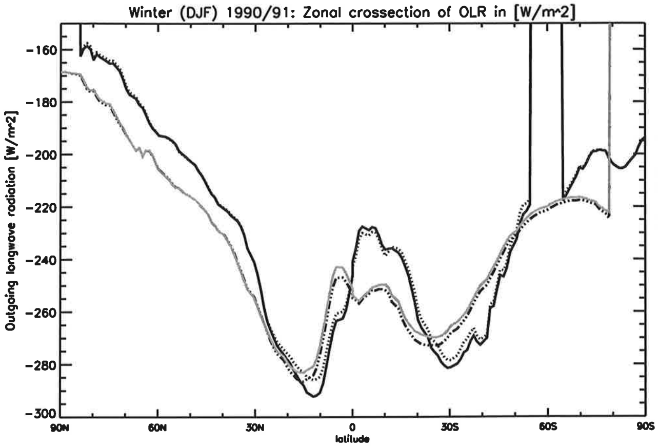
— ERA40 - land ····· Exp. b02d - land -·-·- ERA40 - ocean — Exp. b02d - ocean (a)
