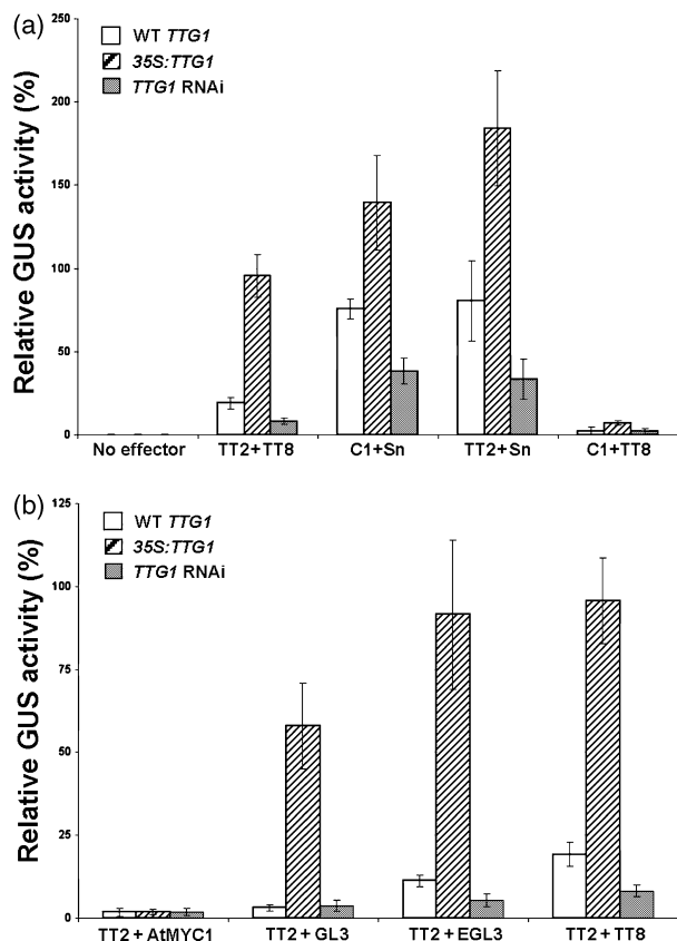
Figure 5. Effect of MYB/bHLH combinations on BAN expression depending on the TTG1 expression level in A. thaliana protoplasts. Relative GUS activity is presented in percentage of the GUS activity generated by a 35S:uidA construct. The effects of different MYB/bHLH combinations were tested with a wild-type TTG1 expression level, TTG1 overexpression, or TTG1 RNAi. Results are mean \pm absolute deviation of eight independent transfection experiments. (a) Comparison of the activity of TT2/TT8 and the maize regulators C1/Sn. (b) Comparison of the activity of the TT2/bHLHs combinations.
