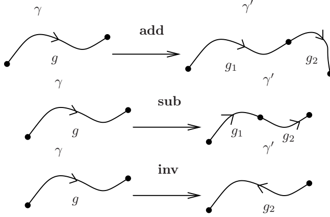
Figure 1: Elementary moves relating ordered graphs
