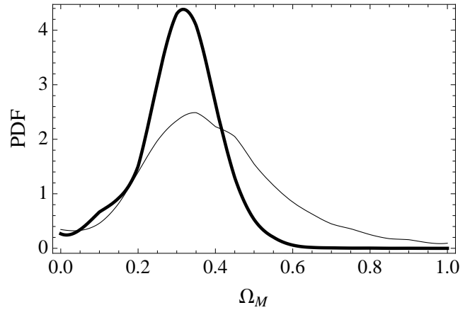
Figure 7. Marginalised posterior probability for \Omega_M as derived from both lensing statistics and time-delays in the case of three lensing events. The thick and the thin lines are for \delta D_{\Delta t}^{\text{Obs}}/D_{\Delta t}^{\text{Obs}} = 10\% or 20\% , respectively.
