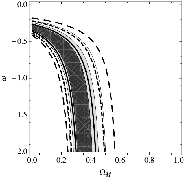
Figure 8. Posterior probability for \Omega_M and \omega as derived from 3 measured time-delays of sources with known redshifts. Grey-shadowed regions are for \delta D_{\Delta t}^{\text{Obs}}/D_{\Delta t}^{\text{Obs}} = 10\% ; thick lines are for \delta D_{\Delta t}^{\text{Obs}}/D_{\Delta t}^{\text{Obs}} = 20\% . Contour values are as in Fig. 5.
