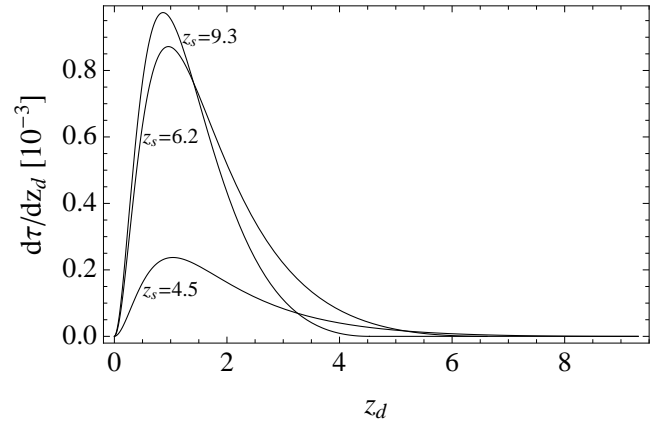
Figure 2. Differential lensing probability for different source redshifts. Probabilities were obtained through Eq. (9). Intrinsic SNR are 400, 12 or 36 for z_s = 4.5, 6.2 or 9.3 , respectively.
