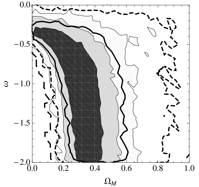
Figure 6. Marginalised posterior probability for \Omega_M and \omega as derived from both lensing statistics and time-delays in the case of 3 lensing events. Regions and contours are as in Fig. 5.
