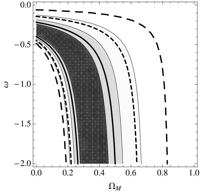
Figure 9. Posterior probability for \Omega_M and \omega as derived from 1 measured time-delay of a source with known redshift. Regions and contours are as in Fig. 8.
