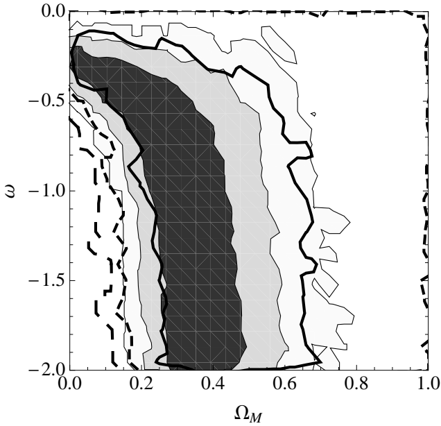
Figure 5. Marginalised posterior probability for \Omega_M and \omega as derived from 3 measured time-delays. Grey-shadowed regions are for \delta D_{\Delta t}^{\text{Obs}}/D_{\Delta t}^{\text{Obs}} = 10\% ; thick (full, dashed or long-dashed) lines are for \delta D_{\Delta t}^{\text{Obs}}/D_{\Delta t}^{\text{Obs}} = 20\% . Contour values are as in Fig. 3.
