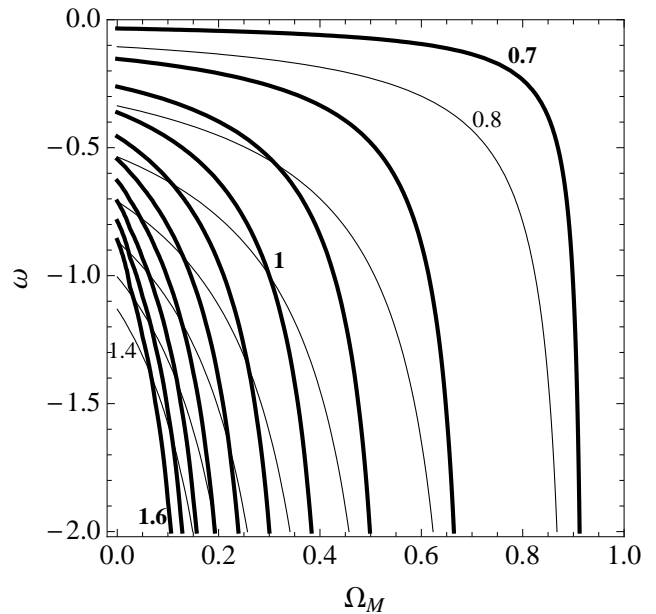
Figure 4. D_{\Delta t}(z_d = 1, z_s = 7) (thick lines) and D_s(z_s = 1) (thin lines) as a function of the cosmological parameters. Values of D_{\Delta t} ( D_s ) are normalised to their value at \Omega_M = 0.3 and \omega = -1 and run from 0.7 (0.8) to 1.6 (1.4) in steps of 0.1. The Hubble constant is fixed to h = 0.7 .
