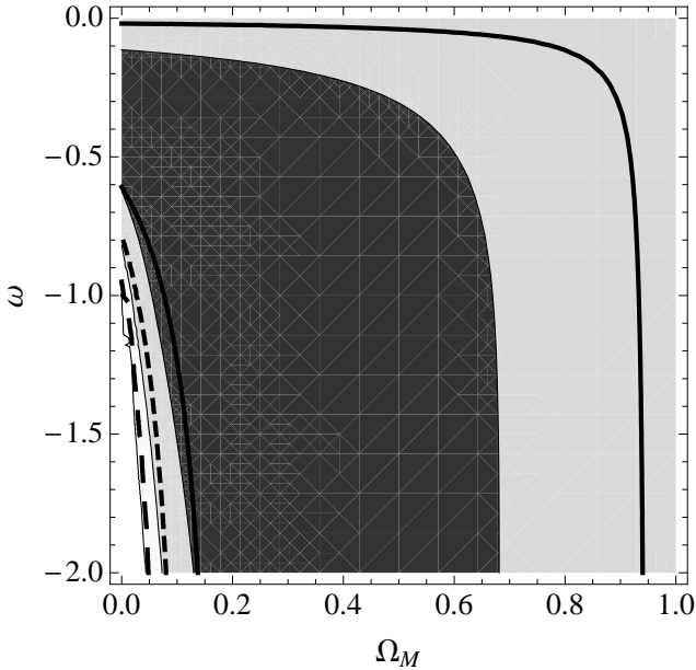
Figure 3. Posterior probability for \Omega_M and \omega as derived from lensing statistics in the case of 3 lensed sources. Grey-shadowed regions or thick contours (full, dashed or long-dashed lines) refer to lensing statistics either exploiting information on lens redshift or assuming z_d to be unknown. Contours are plotted at fraction values \exp(-2.3/2) , \exp(-6.17/2) , and \exp(-11.8/2) of the maximum, which would denote confidence limit region of 1-, 2- and 3- \sigma in a maximum likelihood investigation, respectively.
