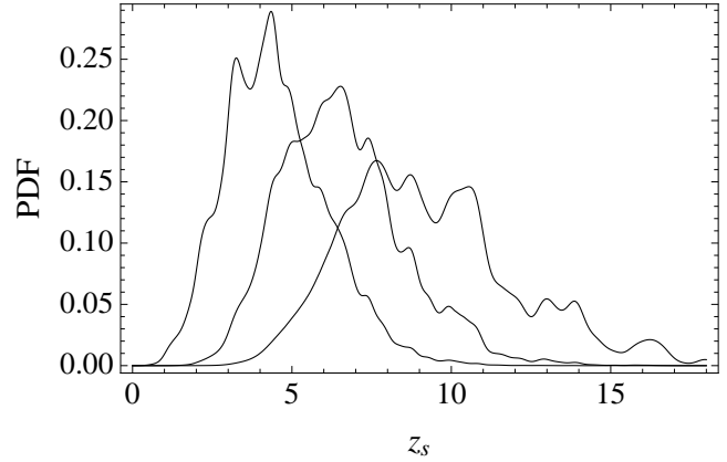
Figure 1. Probability density functions for the redshift of the 3 lensed sources. PDFs have been obtained by repeatedly extracting a triple from the intrinsic redshift distributions of the simulated LISA sources. Each source was weighted by its optical depth to lensing.
