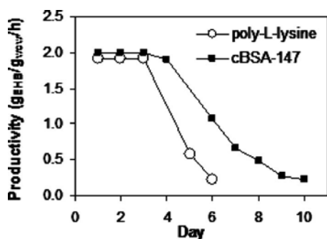
FIG. 8. Sustainability of the coated microreactor (25 mM of EAA, 50 mM IPA, 2 mM Mg 2+ , and 37 °C). cBSA-147 coated cells: 13.5 mg wcw , substrate solution flow rate 18.5 ml/h; PLL coated cells: 8.4 mg wcw , substrate solution flow rate 18.8 ml/h.
