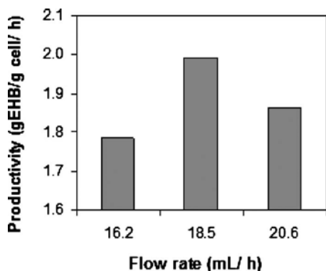
FIG. 7. Productivity of the immobilized cells on a cBSA-147 coated microchannel as function of substrate flow rate. Reaction conditions: 13.5 mg wcw , 25 mM of EAA, 50 mM IPA, 2 mM Mg 2+ , and 37 °C.
