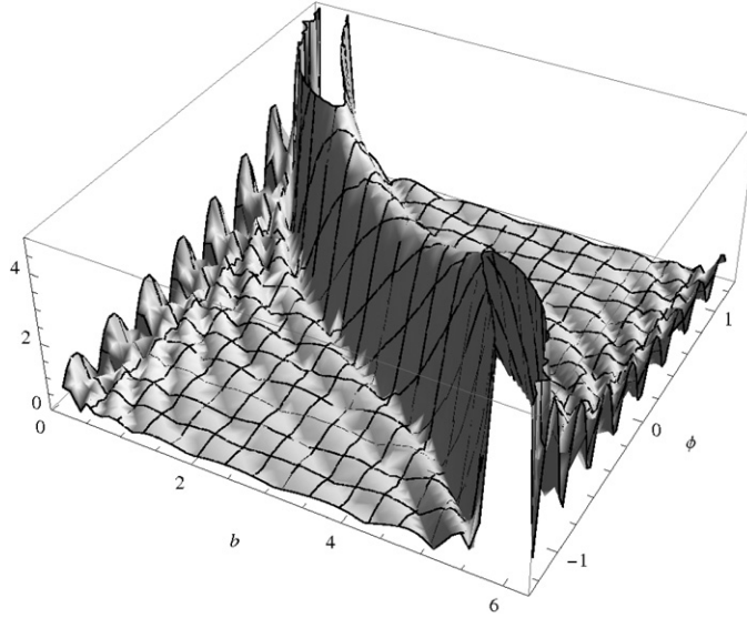
Figure 2. Wave packet |\psi(b, \phi)| in solvable LQC, with A_L(k) = 0 , A_R(k) = e^{-0.01k^2} in (35), where again \nu_0 = 3\pi G = 1 .
