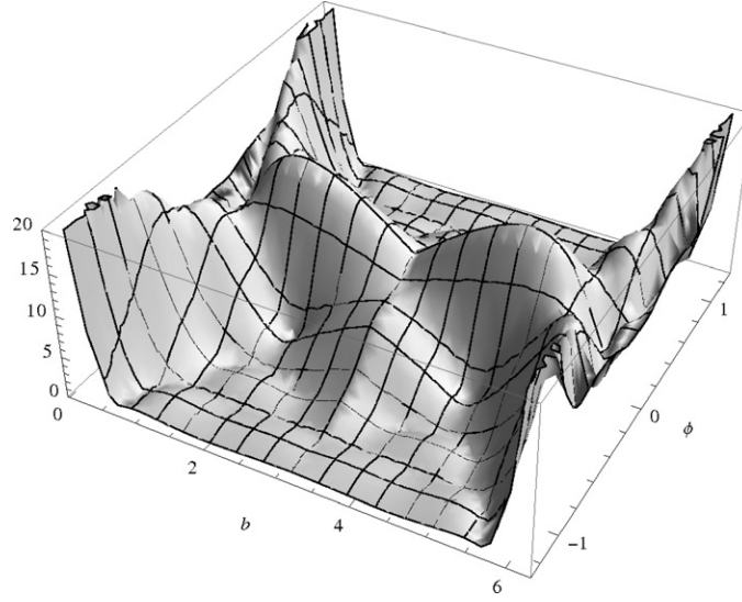
Figure 1. Wave packet |\psi(b, \phi)| formed out of the solutions (44), with \lambda = 0.01 and \nu_0 = 3\pi G = 1 , so that b \in [0, 2\pi) .
