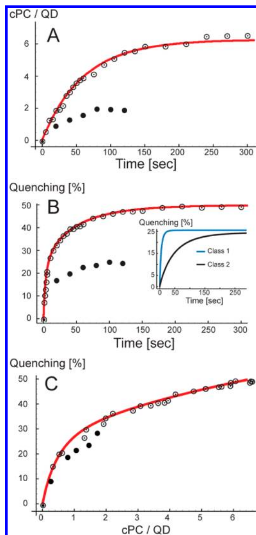
Figure 3. Photoconversion data and fits. Dual-color psQDs were irradiated with 340 \pm 10 nm UV light, irradiance 1.1 \text{ mW cm}^{-2} [ \circ , Data]; [red line, Fit] or 365 nm UV light, irradiance 1.05 \text{ mW cm}^{-2} [ \bullet , Data] for 1–15 s, absorbance and fluorescence spectra were recorded, and then a new pulse was applied. (A) Mean value of cPC molecules per QD as a function of irradiation time. (B) Fluorescence quenching of QD as a function of irradiation time. Inset: Quenching % corresponding to the two classes of acceptor as a function of time: blue line, Class 1; black line, Class 2. (C) Fluorescence quenching of QD as a function of mean value of cPC molecules per QD.
