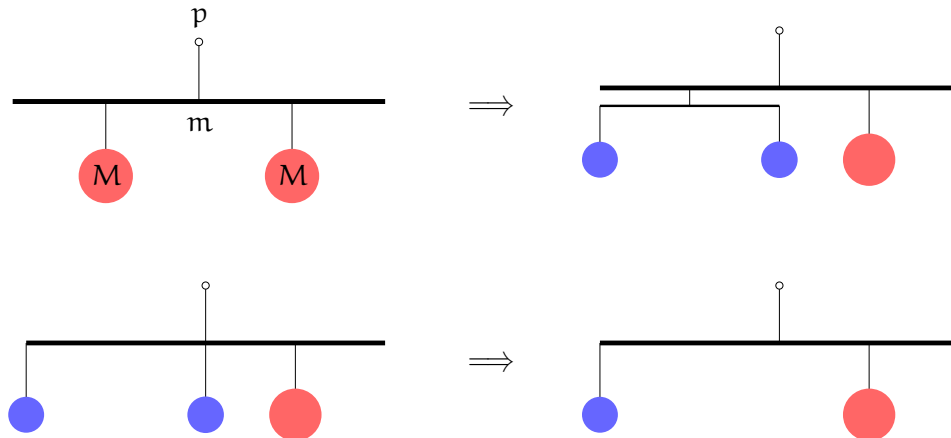
Figure 1: The law of the lever ‘derived’ from alleged symmetry considerations. The step from the upper right (second) to the lower left (third) picture does not follow. The small (blue) balls represent half the mass of the big (red) balls.
