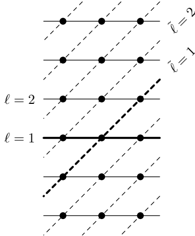
Figure 1: Embedding of the original and dual superconformal symmetries Q = Y^{(1)} , \tilde{Q} = \tilde{Y}^{(1)} into the integrable structure, Y^{(\ell)} or \tilde{Y}^{(\tilde{\ell})} .
