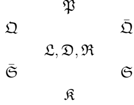
Figure 2: Structure of the superconformal algebra \mathfrak{psu}(2,2|4) . The generators are arranged in the plane according to their charges under two Cartan generators ( \mathfrak{B}, \mathfrak{D} ) which are conserved in commutators.
