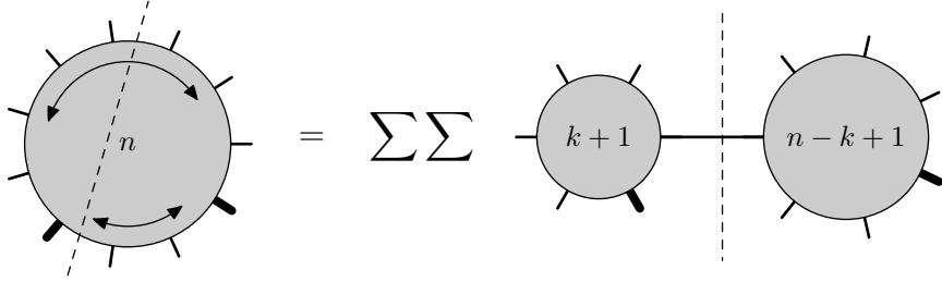
Figure 8: Schematic of the on-shell recursion relation for a general tree-level amplitude. The shifted momenta are denoted by thickened legs and the sum is over the product of subamplitudes which split the shifted legs.
