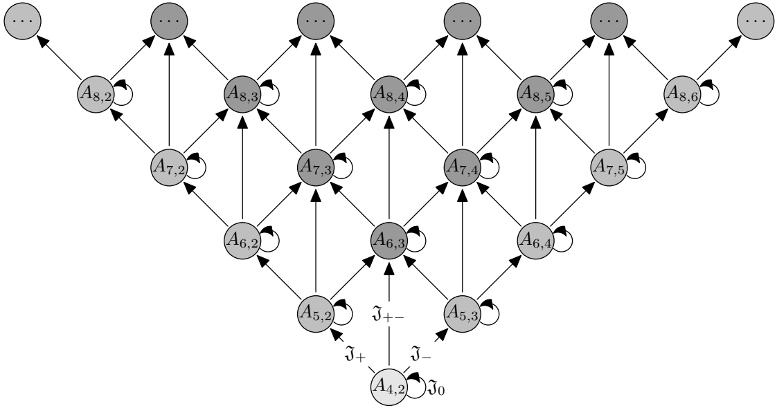
Figure 7: Illustration of the recursive action of the deformed generators.
