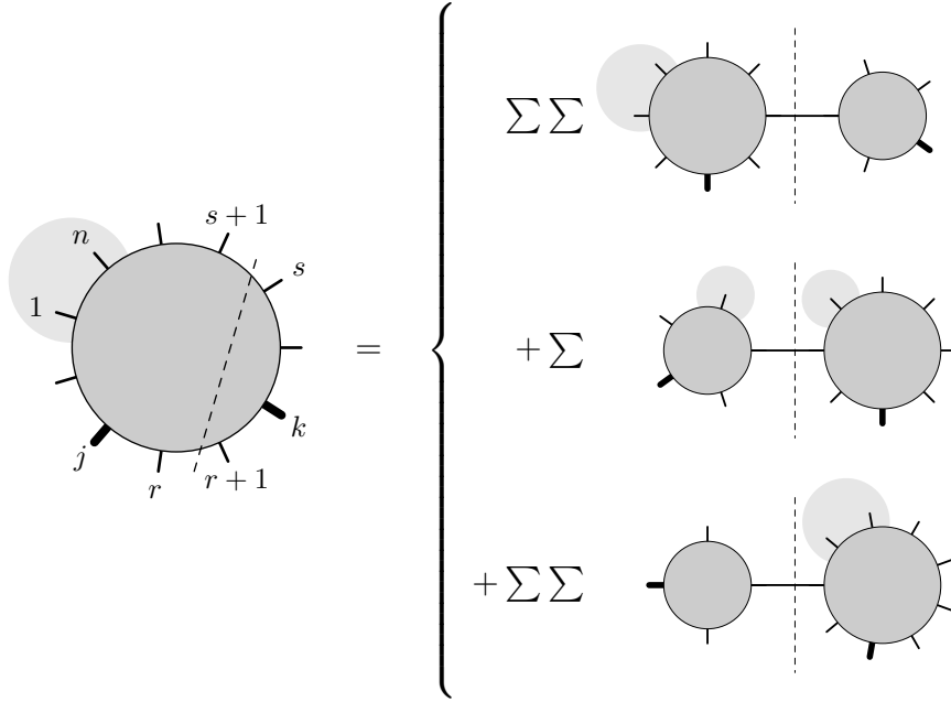
Figure 9: Illustration of the three positions of collinear legs in the recursion relations for the collinear legs chosen to be different than the shifted legs.
