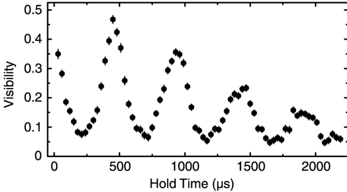
Fig. 5 Visibility of the spatial interference patterns vs. different collisional interaction times t_{hold} . We have been able to observe up to four entangling-disentangling cycles in the experiment. The reduced visibility for longer hold times is mainly caused by a dephasing over the trapped cloud of atoms due to inhomogeneities in the external potentials.
