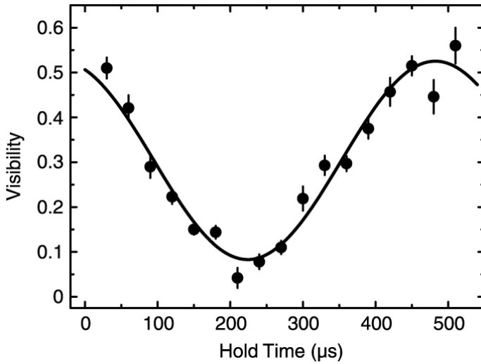
Fig. 3 Visibility of Ramsey fringes vs. hold times on neighbouring lattice sites for the experimental sequence similar to the one displayed in Fig. 1a. The solid line is a sinusoidal fit to the data including an offset and a finite amplitude. Such a sinusoidal behaviour of the visibility vs. the collisional phase shift (determined by the hold time t_{hold} ) is expected for a Mott insulating state with an occupancy of n=1 atom per lattice site 23 . The maximum observed visibility is limited to 55% by inhomogeneities and time dependent fluctuations of the lattice potentials
