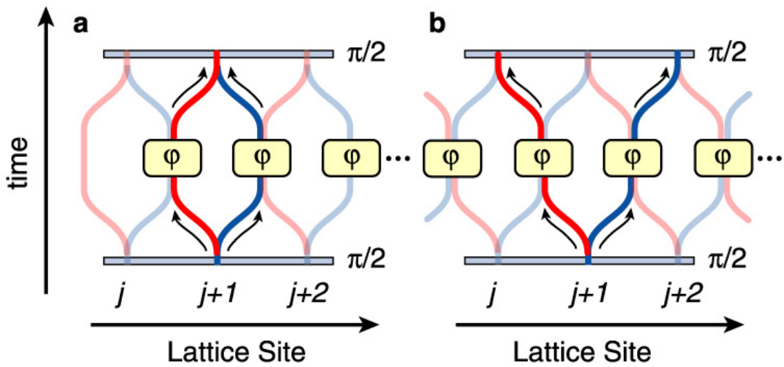
Fig. 1. Schematic multiple quantum gate sequences based on controlled interactions. a A chain of neutral atoms on different lattice sites is first placed in a coherent superposition of two spin states |0\rangle (red) and |1\rangle (blue) with a \pi/2 microwave pulse. Then a spin-dependent transport is used to split the spatial wave packet of an atom and move these two components along two opposite directions depending on their spin state. The wave packets are separated by a lattice period such that each atom is brought into contact with its neighbouring atom. Due to the collisional interaction between the atoms, a phase shift \phi is acquired during a time t_{hold} that the atoms are held on a common lattice site
