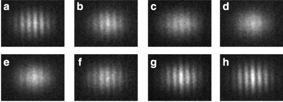
Fig. 4 Spatial interference patterns recorded after applying the multiple quantum gate sequence of Fig. 1b for different collisional interaction times t_{hold} . The different hold times of a 30 \mu s, b 90 \mu s, c 150 \mu s, d 210 \mu s, e 270 \mu s, f 330 \mu s, g 390 \mu s and h 450 \mu s lead to different collisional phase shifts \varphi , ranging from approx. \varphi \approx 0 ( a ) to just over \varphi \approx 2\pi ( h ). The vanishing and reappearance of the interference pattern is caused by the coherent entangling-disentangling dynamics in the many body system due to the controlled collisions between neighbouring atoms. The state selective absorption images were obtained after a time of flight period of 11 ms.
