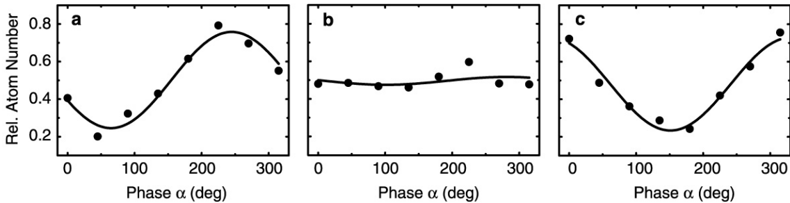
Fig. 2 Experimentally measured Ramsey fringes for different hold times t_{\text{hold}} during which atoms undergo a controlled collisional interaction with their neighbouring atoms. The experimental sequence used is similar to the one in Fig. 1a, where atoms are returned to their original lattice site after the controlled interaction. The hold times t_{\text{hold}} are a 30 \mu\text{s} , b 210 \mu\text{s} and c 450 \mu\text{s} . The relative number of atoms N_{\text{rel}}=N_r/N_{\text{tot}} in the |1\rangle state vs the phase \alpha of the final microwave \pi/2 pulse is measured. A state selective absorption imaging of the
