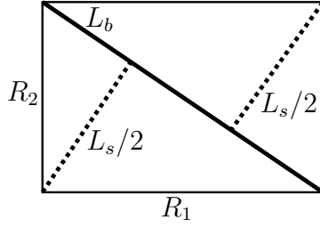
Figure 3: The diagonal brane with length L_b and a string with length L_s that winds perpendicular to the brane around the torus.
