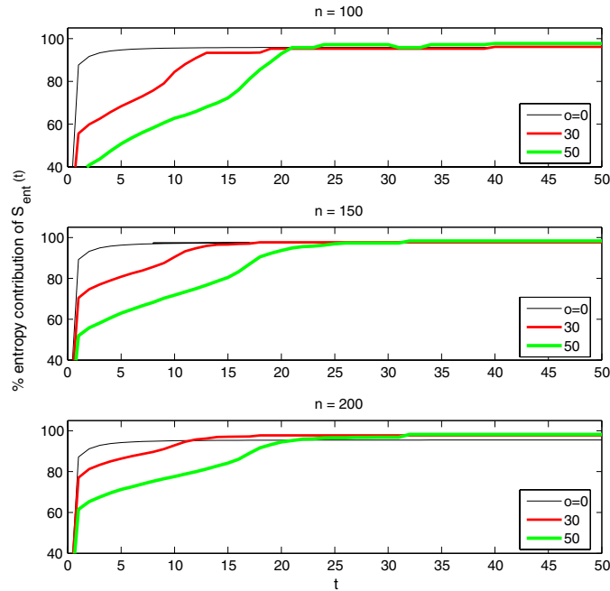
Figure 2. Plot of the percentage contribution of S_{\text{ent}}(t) for the GS and ES. Here again, N = 300 , n = 100, 150 and 200 , and the solid thin curve is for the GS and bold (light) thick curve for o = 30(50) .
