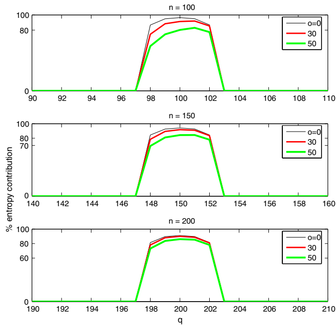
Figure 1. Plot of the percentage contribution to the entropy for the GS and ES as we move the window q - 2 \leq i < q + 2 from q = 2 to q = n , for N = 300 and n = 100, 150 and 200 . The solid thin curve is for the GS o = 0 and the bold (light) thick curve for o = 30(50) .
