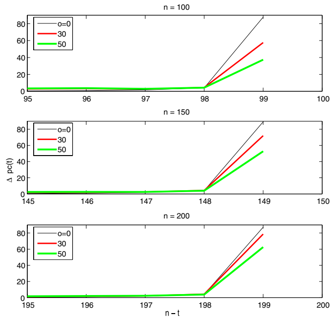
Figure 3. Plot of \Delta pc(t) versus n - t for GS and ES. Here again, N = 300 , n = 100, 150 and 200 , and the solid thin curve is for the GS and bold (light) thick curve for o = 30(50) .
