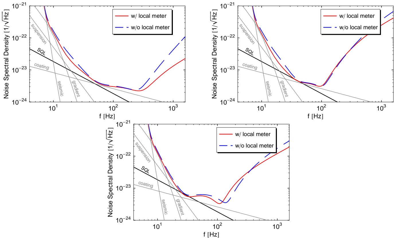
FIG. 4: Noise curves for the scheme with local readout (power of 2 nd carrier fixed to P^{(2)} = 4 kW) and without local readout both optimized for binary systems with total mass M = 2.8 M_{\odot} (upper left), M = 40 M_{\odot} (upper right) and M = 120 M_{\odot} (lower). Special parameters used for optimizations are given in Tab. II and all others in Tab. I. Here classical noise (grey lines) is included. Single contributions of the classical noise are labeled according to their appearance: suspension thermal noise results from the fluctuations in the suspension system; seismic noise is due to motion of the ground; thermal fluctuations in the coating dominates the one in the substrate; gravity gradient noise accounts for time-changing Newtonian gravitational forces.
