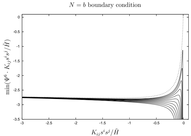
FIG. 3: Values of \Psi^6 \cdot K_{ij}s^i s^j/\tilde{H} and \theta_{(\hat{k})}/\tilde{H} , for boundary conditions K_{ij}s^i s^j = \lambda , b = N and \Omega_o = 0, 0.10, 0.11, 0.12, \dots, 0.20 . Curves depart from the spherically symmetric case (dotted curve corresponds to \Omega_o = 0 ) as the rotating parameter increases. Solutions exist for every prescribed \theta_{(\hat{k})} and are unique.
