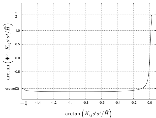
FIG. 2: Numerical analysis of condition (15). Values of \theta_{(\hat{k})}/\tilde{H} = K_{ij} s^i s^j/\tilde{H} and \Psi^6 \cdot K_{ij} s^i s^j/\tilde{H} in the spherically symmetric case, after compactification by means of the arctan function.
