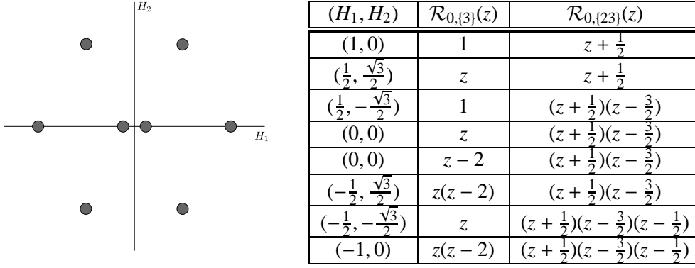
Figure 1: Polynomial structure of the \mathcal{R} -operators using the normalization in [10].
