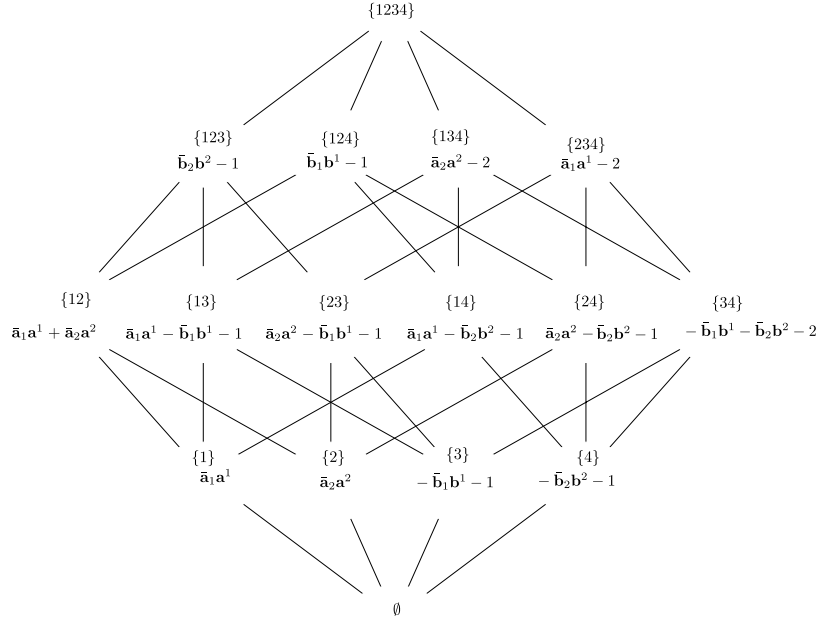
Figure 2: Hasse diagramm for \mathfrak{su}(2, 2) including the shifted weights of the subalgebra \hat{\mathcal{L}}_1^I - \gamma according to (C.18).
