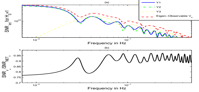
FIGURE 3. (a) SNR of v_+ and Y^{(t)} vs f , (b) SNR_{v_+} / SNR_{Net} vs f for tracking \{\theta_B, \phi_B\} = \{60^\circ, 200^\circ\} .
