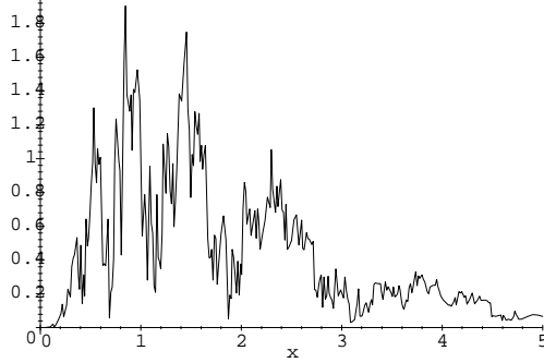
FIGURE 2. a_n = n^{-1}, b_n = n^2, k = 1, \lambda = 0.5, m = 50
