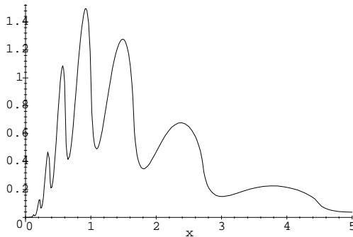
FIGURE 1. a_n = n^{-2}, b_n = n, k = 1, \lambda = 0.5, m = 200
