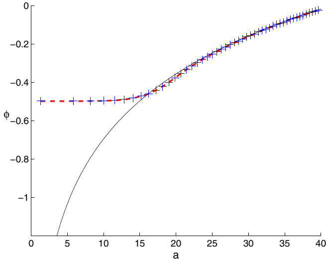
FIG. 3 (color online). Comparison of evolution via the quantum constraint (+ line), ET-I and ET-II (dashed line), and classical theory (solid line) for J = 500 , P_\phi = 100l_p . Classical theory breaks down for a < a_* , whereas ET-I and ET-II are valid until a_0 .
