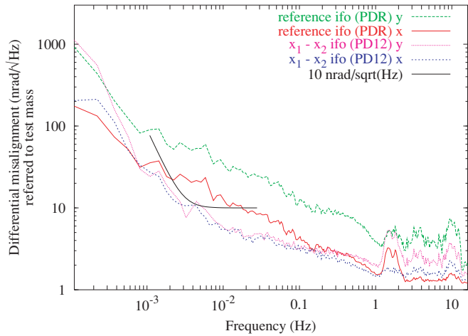
Figure 4. Linear spectral density of the DWS alignment measurements (see the text).
