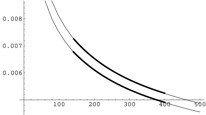
Figure 5: A fit of \max|U_{mn}^{22}| for even (bottom curve) and odd levels. For even levels we get a = -0.0026, b = 0.027, c = 0.21 . For odd levels we get a = -0.0012, b = 0.031, c = 0.26 . Again, the data seems consistent with the vanishing of U_{22} .
