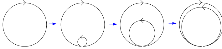
Figure 2: Using zig-zag symmetry and shape independence to show that \langle \frac{1}{N} \text{tr} W(C) \rangle = 1 . This assumes that shape independence still holds when cusps are introduced. An argument which avoids this assumption relies on properties of the chiral ring.
