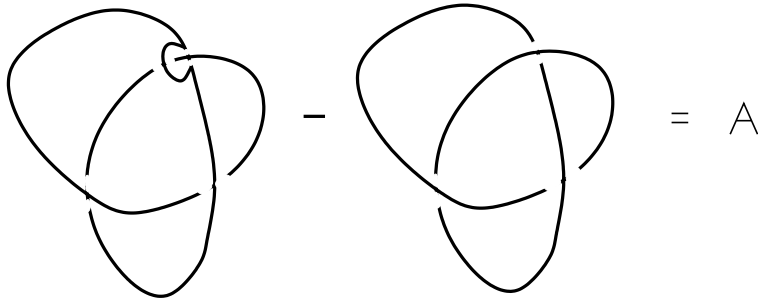
Figure 1: (Almost) loop equation.
