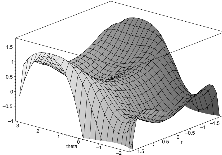
Figure 1: For this plot we have chosen a = 5 , b = -1 , c = 0.1 . It shows one AdS minimum at (r, \theta) = (0, -\frac{\pi}{2}) , a flat space vacuum at (r, \theta) = (0, \frac{\pi}{2}) and in-between there is a deSitter saddle point.
