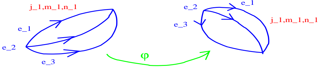
Figure 10: Action of Spatial Diffeomorphisms on SNW's
