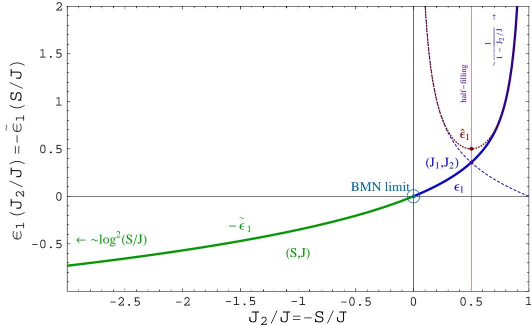
Figure 1: The leading order correction to the energy \epsilon_1 for the folded string solution. The region J_2/J > 0 correspond to the (J_1, J_2) case, whereas J_2/J < 0 correspond to the (S, J) case with S/J = -J_2/J and energy \tilde{\epsilon}_1 = -\epsilon_1 . We also plot a mirror image under the symmetry J_1 \leftrightarrow J_2 (dashed) and the energy of the circular string \hat{\epsilon}_1 (dotted).
