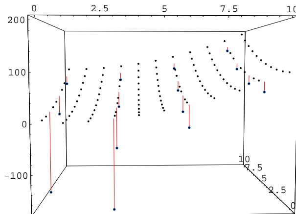
Fig. 2: This graph shows the dispersion relation for \theta = \frac{1000}{3001} .
