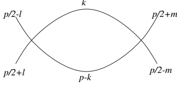
Fig. 3: The fish graph
