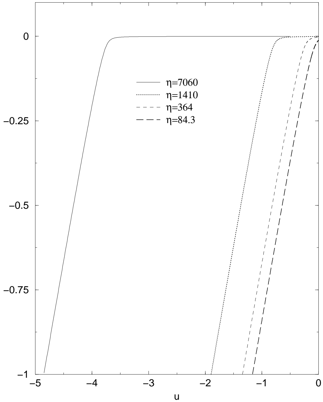
FIG. 5. \hat{\tau}(u) versus u for 4 values of \eta .
