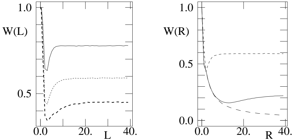
Fig. 3 D = 4 Susy Wilson loops (a) Square of side length L with N = 2, 4, 8 (top to bottom) (b) square, regular 16-gon and 64-gon enclosed in circle of radius R with N = 4 .
