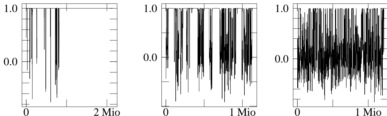
Fig. 1 Autocorrelation functions versus Monte Carlo time for the SU(2) bosonic integral with, from the left, D = 3, 4, 5 .
