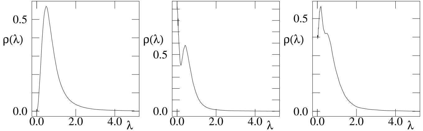
Fig. 2 Eigenvalue (half-)densities for susy D = 4 , from the left, N = 2, 3, 4
