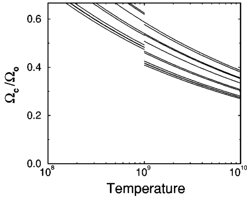
FIG. 1. Temperature dependence of the critical angular velocities of 1.4M_\odot neutron stars constructed with a number of realistic equations of state.
