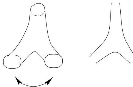
Figure 1: World-sheet diagrams for closed resp. open string interaction. Having assigned vertex operators to the legs, they can be read as structure constants for the multiplication of two operators, projected on the third channel. In the closed string case, the in-coming operators can be interchanged with the help of world-sheet diffeomorphisms, while the ordering of open string vertices is fixed up to cyclic permutations.
