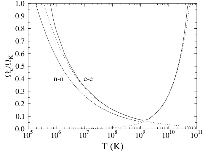
Fig. 1. Critical angular velocity for the onset of the r -mode instability as a function of temperature (for a 1.5 M_\odot neutron star model). The solid line corresponds to the O(\Omega^2) result using superfluid ( e^- - e^- ) shear viscosity, and Sawyer's (1989) estimate for the bulk viscosity. Dotted lines are lowest order approximations, while the dashed line corresponds to normal matter ( n - n ) shear viscosity.
