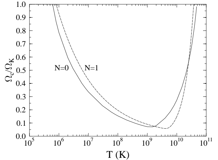
Fig. 2. Critical angular velocity for the onset of the r -mode instability as a function of temperature (for a 1.5 M_\odot neutron star model). The present uniform density result ( N = 0 ) is compared to the critical curve for the equation of state used in Andersson et al. (1998), ( N = 1.0 polytrope). The minimum value of \Omega_c/\Omega_K is roughly the same, and the effect of the equation of state is mainly to shift the critical curve to different temperatures.
