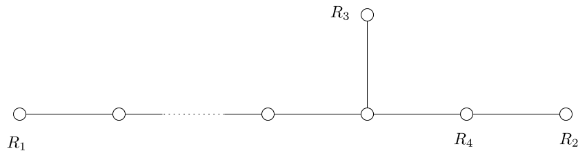
Figure 1: Dynkin indices of some reducibility representations.
