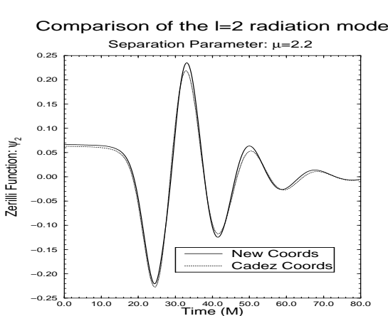
Fig. 4: \ell = 2 waveform comparison between the class I and Čadež grids.
