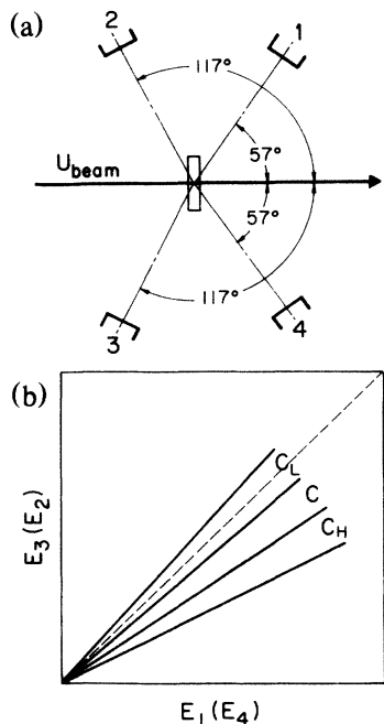
FIG. 1. (a) Experimental arrangement. The Th target is placed at 90^\circ to the U beam. The Ge detectors (1-4) were placed 13 cm from the target at the angles shown. (b) Schematic sketch of the windows chosen to select the particular Doppler velocities: for C , \beta = \beta_{c.m.} , for C_L , \beta = 0 , and for C_H , \beta = 2\beta_{c.m.} . The photon energies are denoted by E_i where i is the detector number in (a).
