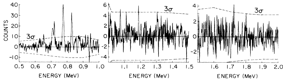
FIG. 3. Difference spectrum between Figs. 2(a) and 2(d). The dashed lines correspond to statistical 97% confidence limits (3 times the standard deviation) for a 4-keV-wide photon line. The expected \gamma\gamma line(s) should lie in the 1.5–1.8-MeV energy interval.
