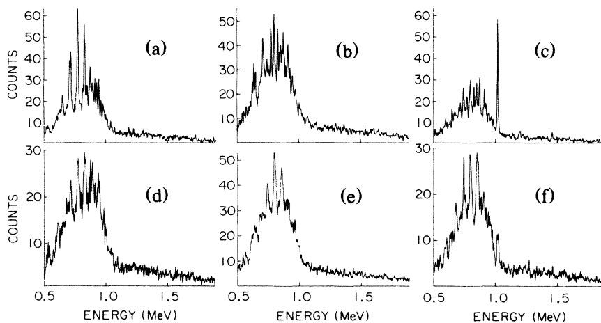
FIG. 2. Summed-energy photon spectra in the Ge detectors shown in Fig. 1(a). Spectra (a), (b), and (c) correspond to 180^\circ (c.m.) correlated detector pairs (1,3) and (2,4), and to windows C , C_H , and C_L , respectively. Spectra (d), (e), and (f) correspond to 60^\circ correlated detector pairs (1,2) and (3,4), and to windows C , C_H , and C_L , respectively. The origin of the line structures is discussed in the text.
