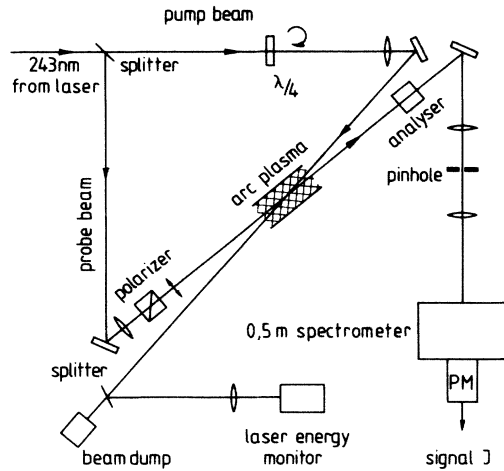
FIG. 1. Experimental setup.
