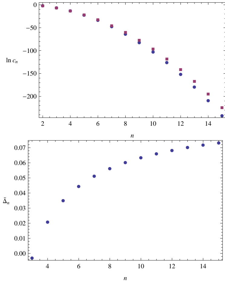
Figure 1: Top panel: the coefficients \ln c_n^{\text{exact}} (dots) and \ln c_n (squares) of the exact and diffusing series, respectively. Bottom panel: \tilde{\Delta}_n \equiv |\ln c_n - \ln c_n^{\text{exact}}| / |\ln c_n^{\text{exact}}| .
