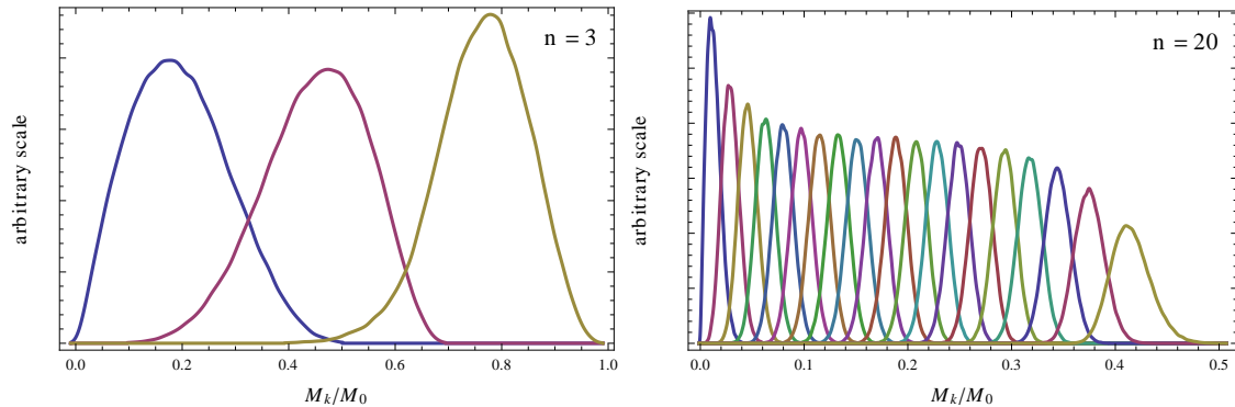
Figure 1: Distribution of the \mathcal{M}_R eigenvalues M_k according to the linear measure from Eq. (23) with the boundary constraint \sum_{k=1}^n M_k^2 \leq M_0^2 .
