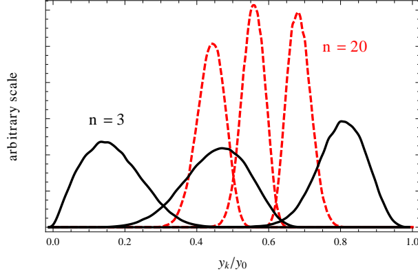
Figure 2: Distribution of the singular values y_k of the Yukawa matrix according to the linear measure from Eq. (24) for n = 3 (black) and n = 20 (red/dashed) with the boundary constraint \sum_{k=1}^3 y_k^2 \leq y_0^2 .
