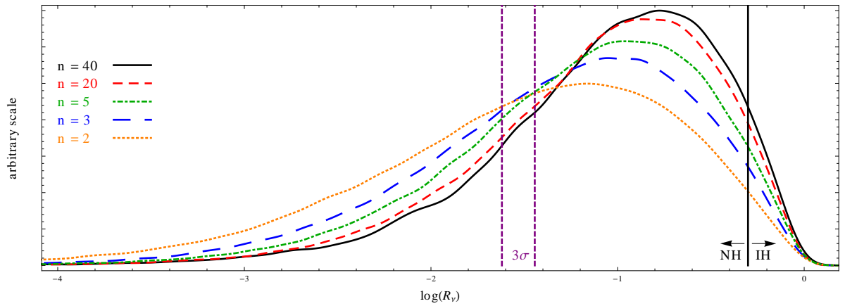
Figure 3: \log_{10}[R_\nu] \equiv \log_{10} [(m_2^2 - m_1^2)/(m_3^2 - m_1^2)] for various n . The purple/dashed vertical lines indicate the 3\sigma range for R_\nu \simeq 0.03 [28] (for NH). The black vertical line divides the NH and IH solutions.
