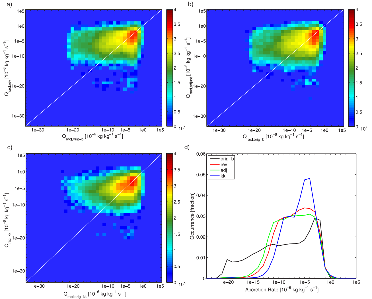
Figure 2. Six-hourly joint-histograms of in-cloud accretion rates from all model levels, (a) untuned version of new scheme ( rev ) against the original scheme ( orig-b ), (b) retuned version of the new scheme ( adjust ) against the original scheme ( orig-b ) and (c) an alternative parameterization ( kk ) against the original scheme ( orig-kk ). (d) Distribution of in-cloud accretion rates calculated by the original scheme ( orig-b ), the untuned ( rev ) and retuned ( adj ) version of the new scheme as well as by an alternative autoconversion parameterization ( kk ) from all model levels of one year.
