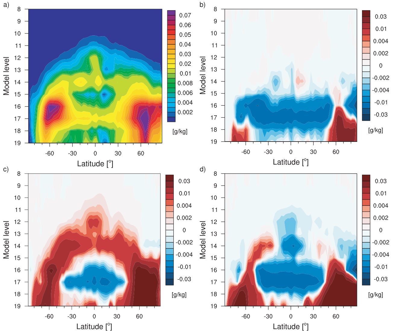
Figure 3. (a) Vertical distribution of zonal annual mean cloud liquid water calculated by the original scheme ( orig-b ), (b) untuned version of the new scheme ( rev ) minus the original scheme ( orig-b ), (c) retuned version of the new scheme ( adjust ) minus the original scheme ( orig-b ) and (d) an alternative parameterization ( kk ) minus the original scheme ( orig-b ).
