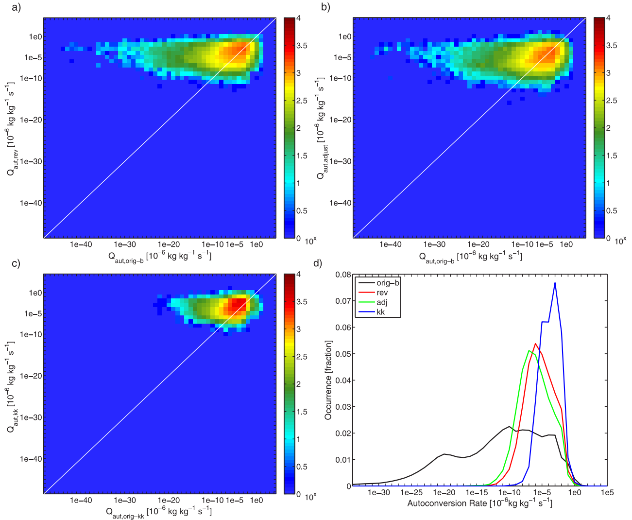
Figure 1. Six-hourly joint-histograms of in-cloud autoconversion rates from all model levels, (a) untuned version of new scheme ( rev ) against the original scheme ( orig-b ), (b) retuned version of the new scheme ( adjust ) against the original scheme ( orig-b ) and (c) an alternative parameterization ( kk ) against the original scheme ( orig-kk ). (d) Distribution of in-cloud autoconversion rates calculated by the original scheme ( orig-b ), the untuned ( rev ) and retuned ( adj ) version of the new scheme as well as by an alternative autoconversion parameterization ( kk ) from all model levels of one year.
