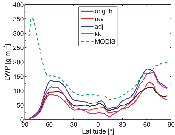
Figure 4. Comparison of the zonal annual mean of LWP simulated by the original autoconversion ( orig-b ), and the untuned ( rev ) and retuned ( adj ), and untuned ( kk ) version of the new autoconversion scheme as well as the column liquid cloud water derived from MODIS satellite data.
