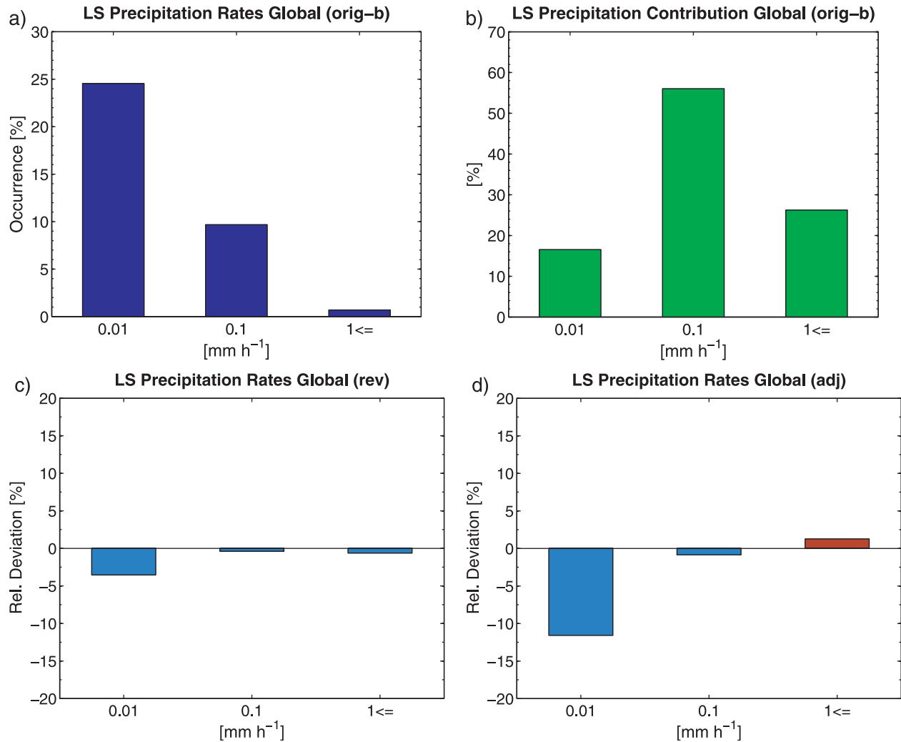
Figure 5. Global large-scale precipitation rates at the surface: (a) occurrence of precipitation rates by categories in the control experiment [%], (b) contribution of categories to the total amount [%] and deviation of occurrence [%] in the (c) untuned and (d) retuned experiment from the control experiment.
