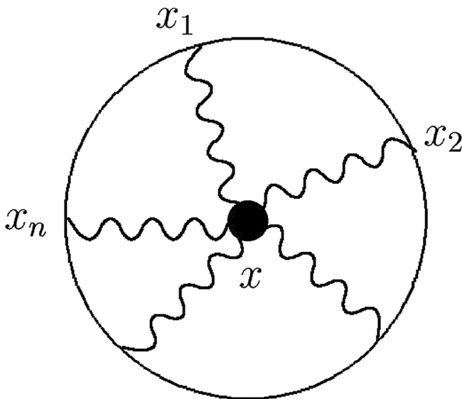
FIG. 1. Witten diagram in twistor space.
