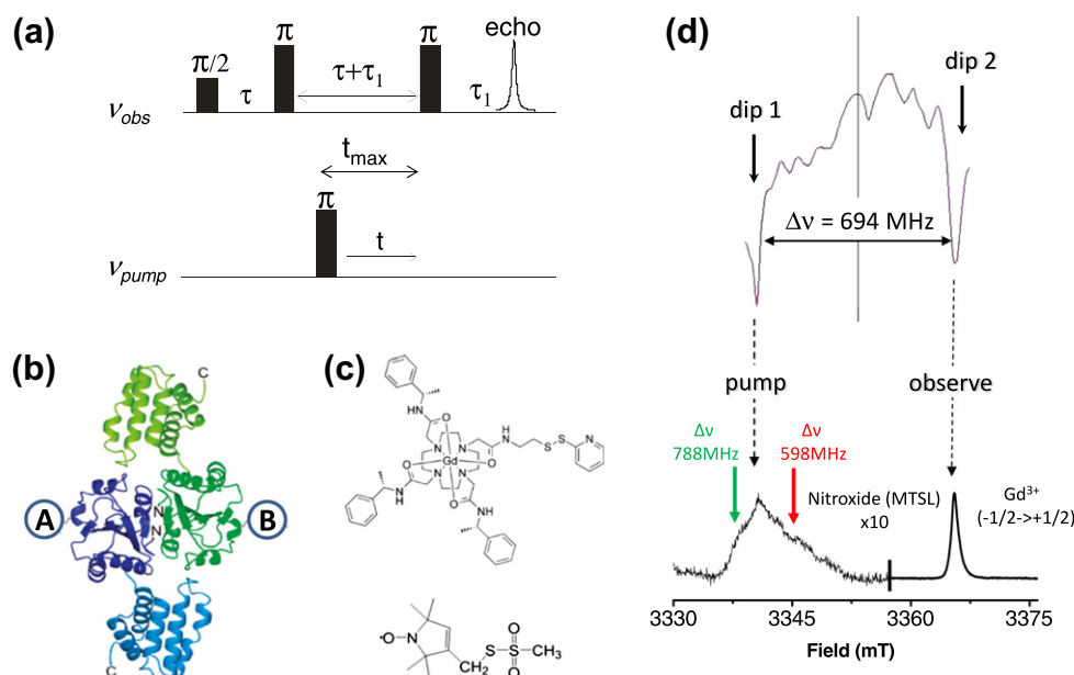
Fig. 1. Experimental setup. (a) 4-pulse DEER pulse sequence used. (b) Structure of the ERp29 protein dimer (PDB ID 2QC7) [33]. The spin labeling positions (S114C) are identified by circles. (c) The Gd^{3+} C1 tag (top) and MTSL tag (bottom) used to spin-label the protein. (d) Characteristic tuning curve showing the two modes of the resonator separated by 694 MHz. This setup was used to apply the pump pulse at the frequency of the g_y component of the nitroxide spectrum. The modes excited in the resonator are TE_{012} (dip 1) and TE_{012-\phi_0} (dip 2). The subscript “ -\phi_0 ” of the second mode indicates the “zero” phase shift between fields in the neighboring resonance cells of the resonator. The mode is a combination of two cylindrical TE_{011} half-wave alternations oscillating in phase in two different cells. The echo-detected EPR spectrum of the statistically labeled ERp29 protein dimer is shown below. Experimental parameters: MW frequency 93.7 GHz; \pi/2 and \pi pulse durations of 40 ns and 80 ns, respectively; \tau = 284 ns; T = 10 K; repetition time 11 ms. Different phase corrections were needed in the two parts of the spectrum to represent both the nitroxide and Gd^{3+} spectrum as absorption lines. All experiments were performed on a Bruker ElexSys E 680 spectrometer (MPLbc, Göttingen) (see Section 4).
